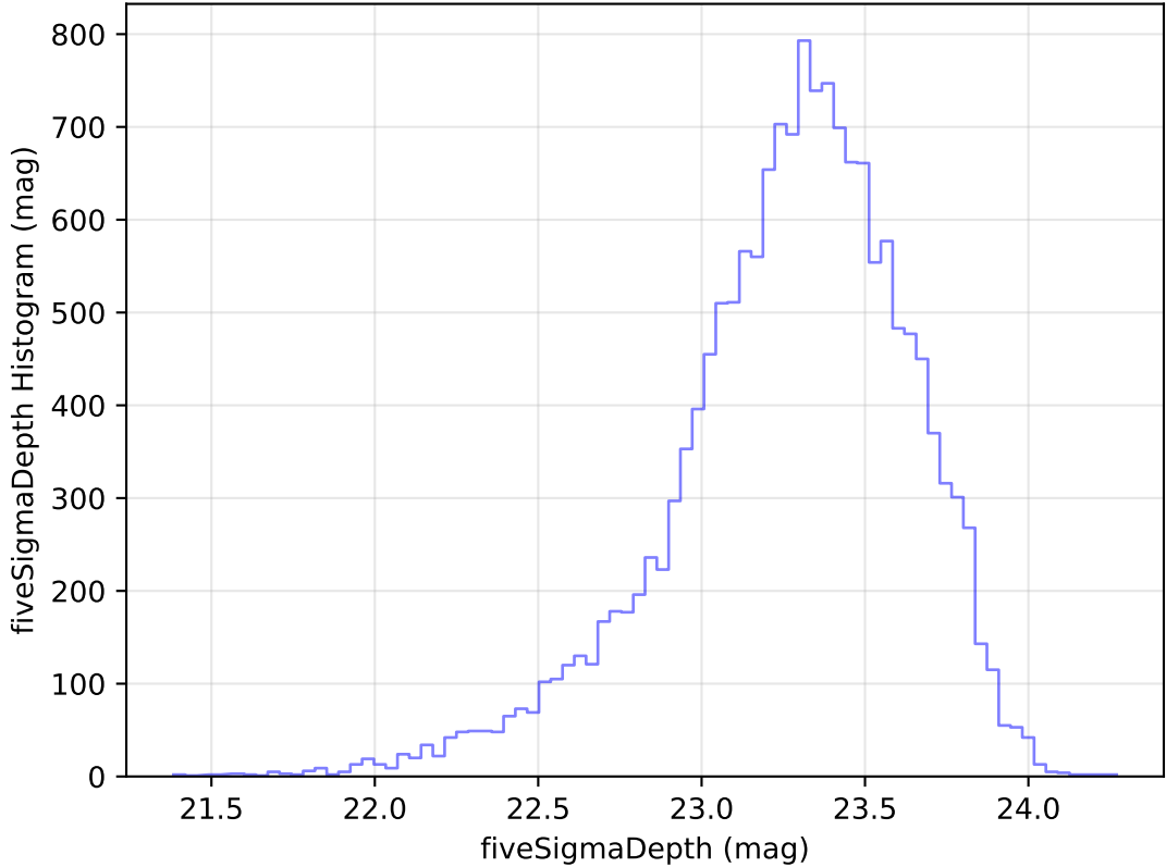
too_elab_heavy_r128_d3_gz_v3.4_10yrs Yr 1 u band: fiveSigmaDepth Histogram
