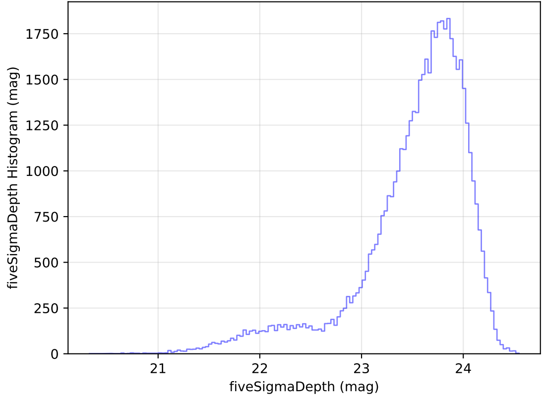
too_elab_heavy_r128_d3_gz_v3.4_10yrs Yr 1 i band: fiveSigmaDepth Histogram
