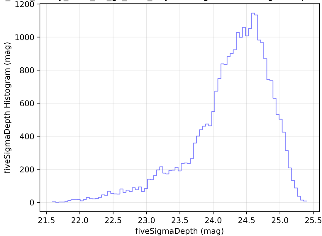
too_elab_heavy_r128_d3_gz_v3.4_10yrs Yr 1 g band: fiveSigmaDepth Histogram
