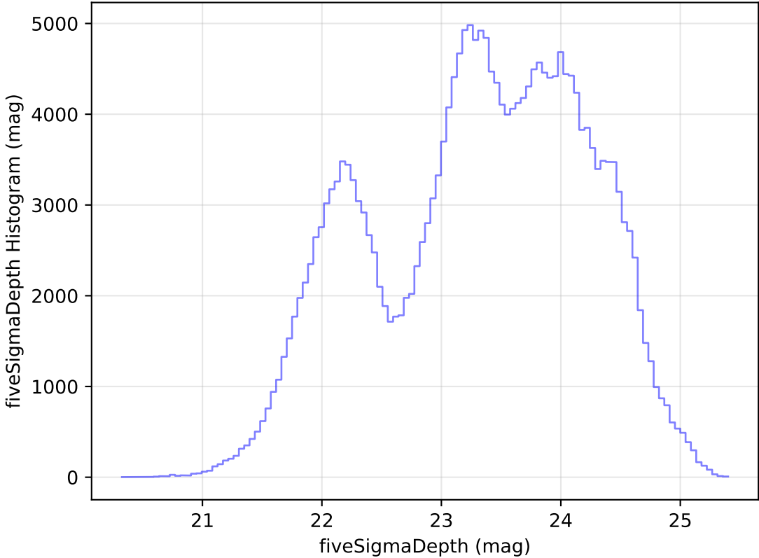
too_elab_heavy_r128_d3_gz_v3.4_10yrs Yr 1 all bands: fiveSigmaDepth Histogram
