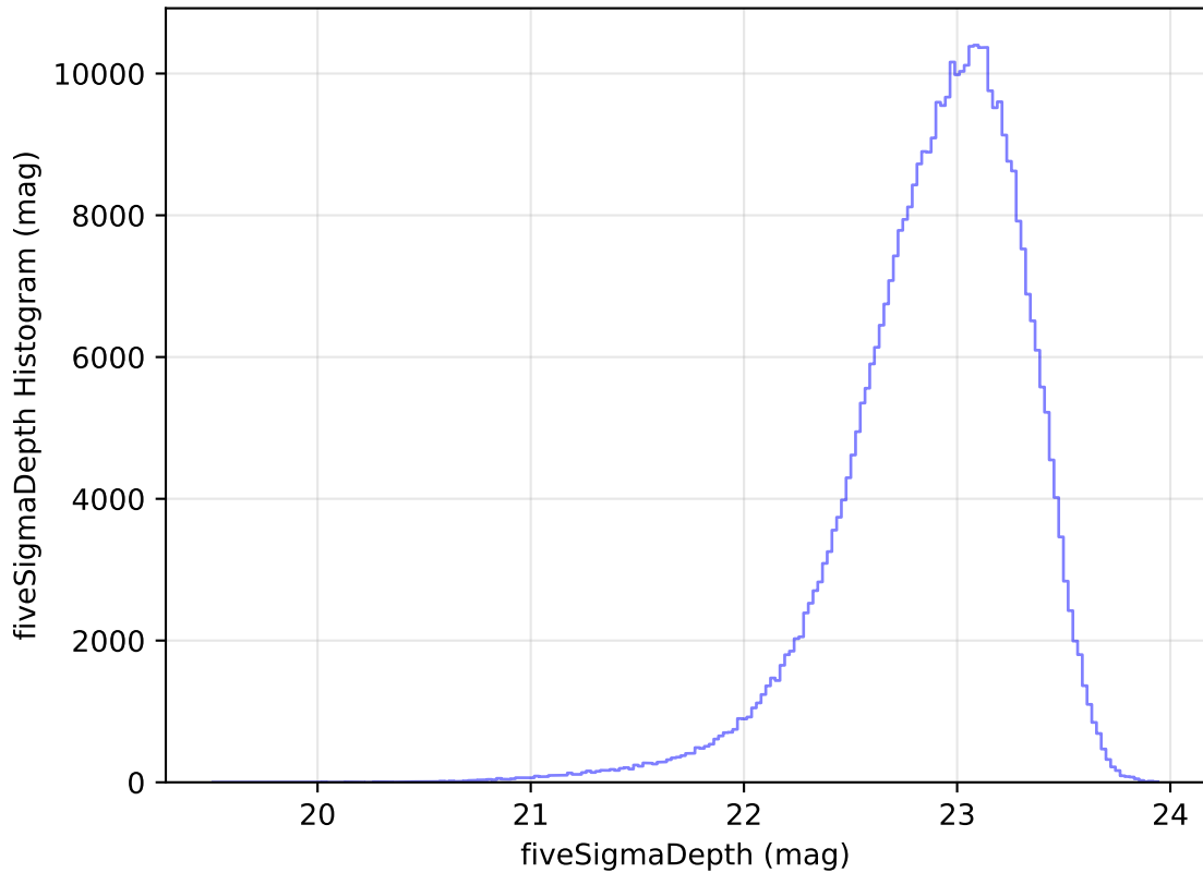
too_elab_heavy_r128_d3_gz_v3.4_10yrs WFD z band: fiveSigmaDepth Histogram
