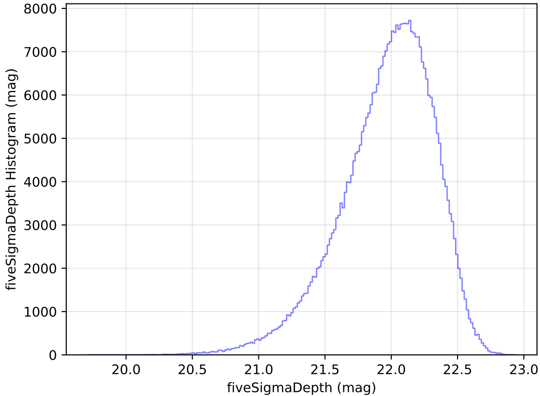
too_elab_heavy_r128_d3_gz_v3.4_10yrs WFD y band: fiveSigmaDepth Histogram
