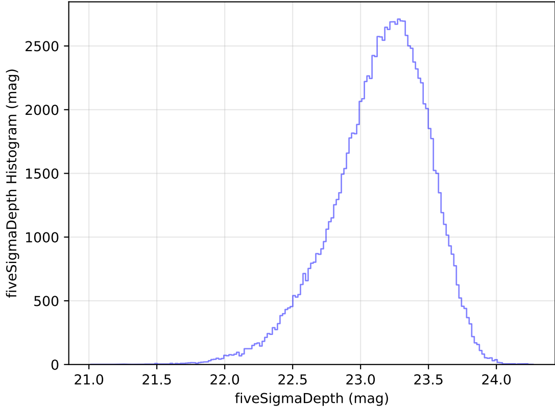
too_elab_heavy_r128_d3_gz_v3.4_10yrs WFD u band: fiveSigmaDepth Histogram
