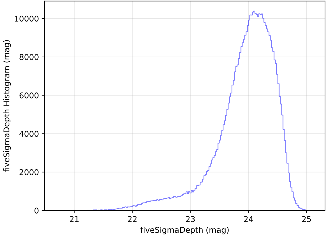
too_elab_heavy_r128_d3_gz_v3.4_10yrs WFD r band: fiveSigmaDepth Histogram
