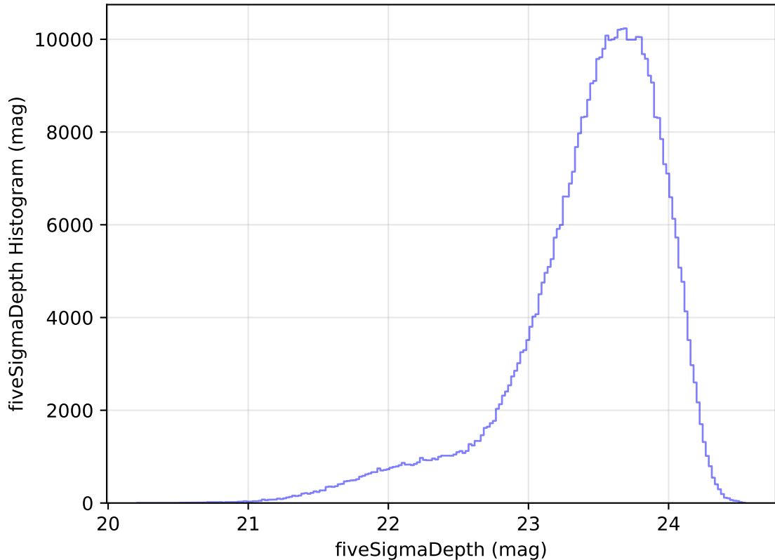
too_elab_heavy_r128_d3_gz_v3.4_10yrs WFD i band: fiveSigmaDepth Histogram
