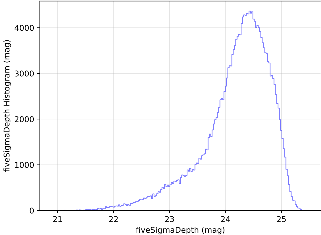
too_elab_heavy_r128_d3_gz_v3.4_10yrs WFD g band: fiveSigmaDepth Histogram
