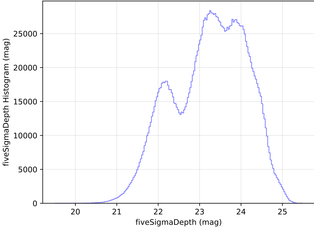
too_elab_heavy_r128_d3_gz_v3.4_10yrs WFD all bands: fiveSigmaDepth Histogram
