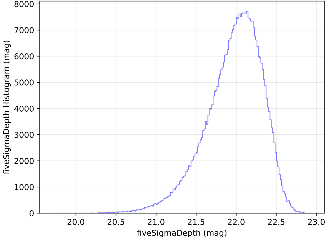
too_elab_heavy_r128_d3_gz_v3.4_10yrs All sky y band: fiveSigmaDepth Histogram
