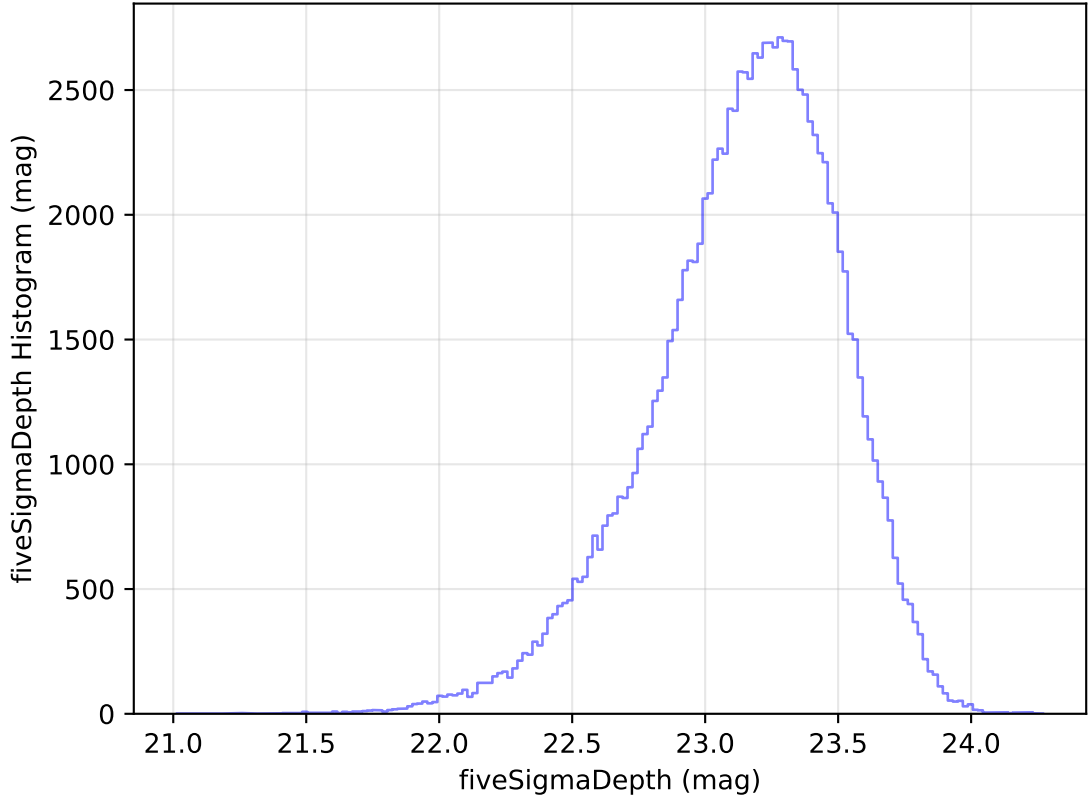
too_elab_heavy_r128_d3_gz_v3.4_10yrs All sky u band: fiveSigmaDepth Histogram
