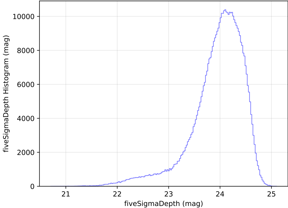
too_elab_heavy_r128_d3_gz_v3.4_10yrs All sky r band: fiveSigmaDepth Histogram
