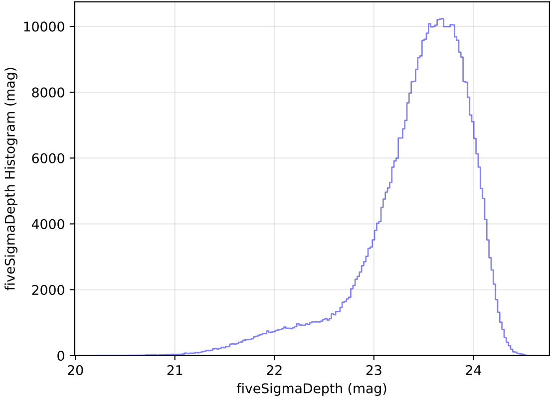
too_elab_heavy_r128_d3_gz_v3.4_10yrs All sky i band: fiveSigmaDepth Histogram
