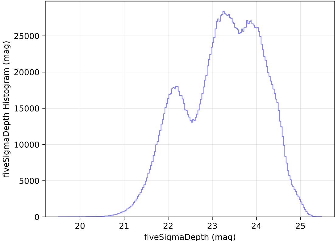
too_elab_heavy_r128_d3_gz_v3.4_10yrs All sky all bands: fiveSigmaDepth Histogram
