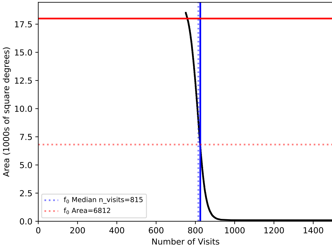
too_elab_heavy_r128_d3_gz_v3.4_10yrs WFD: fO
