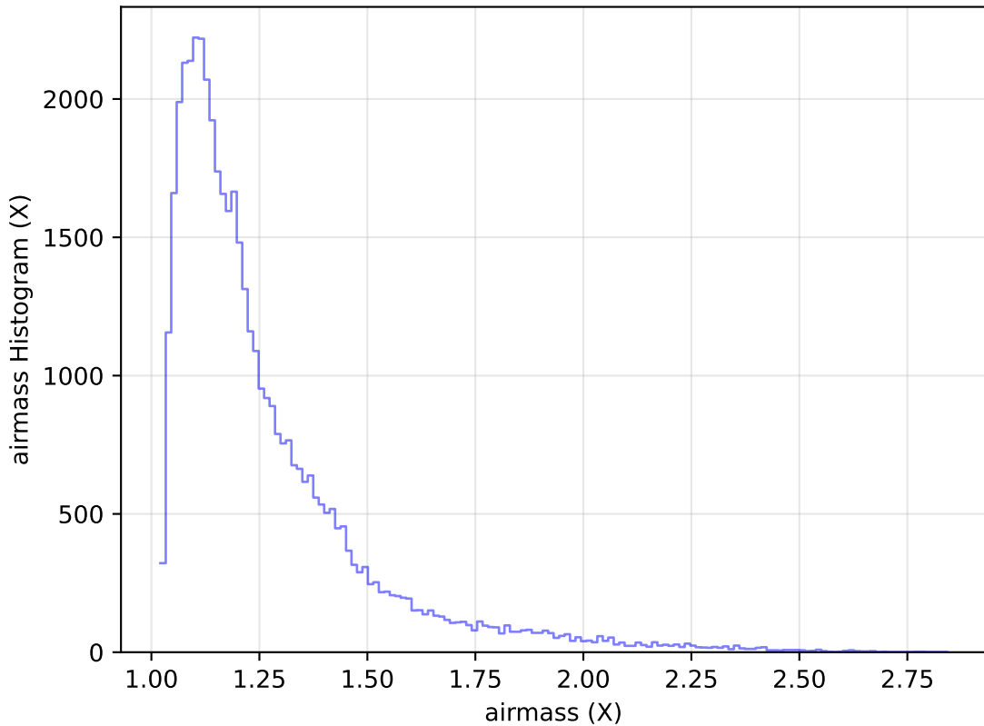
too_elab_heavy_r128_d3_gz_v3.4_10yrs Yr 1 y band: airmass Histogram
