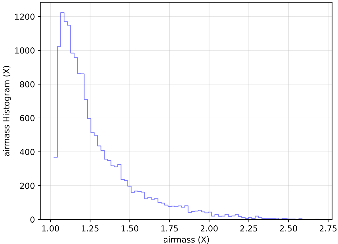
too_elab_heavy_r128_d3_gz_v3.4_10yrs Yr 1 u band: airmass Histogram
