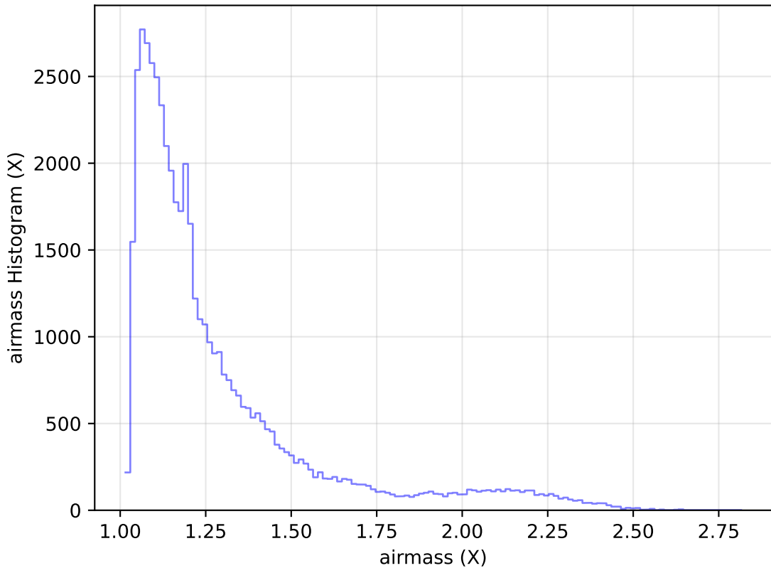
too_elab_heavy_r128_d3_gz_v3.4_10yrs Yr 1 r band: airmass Histogram
