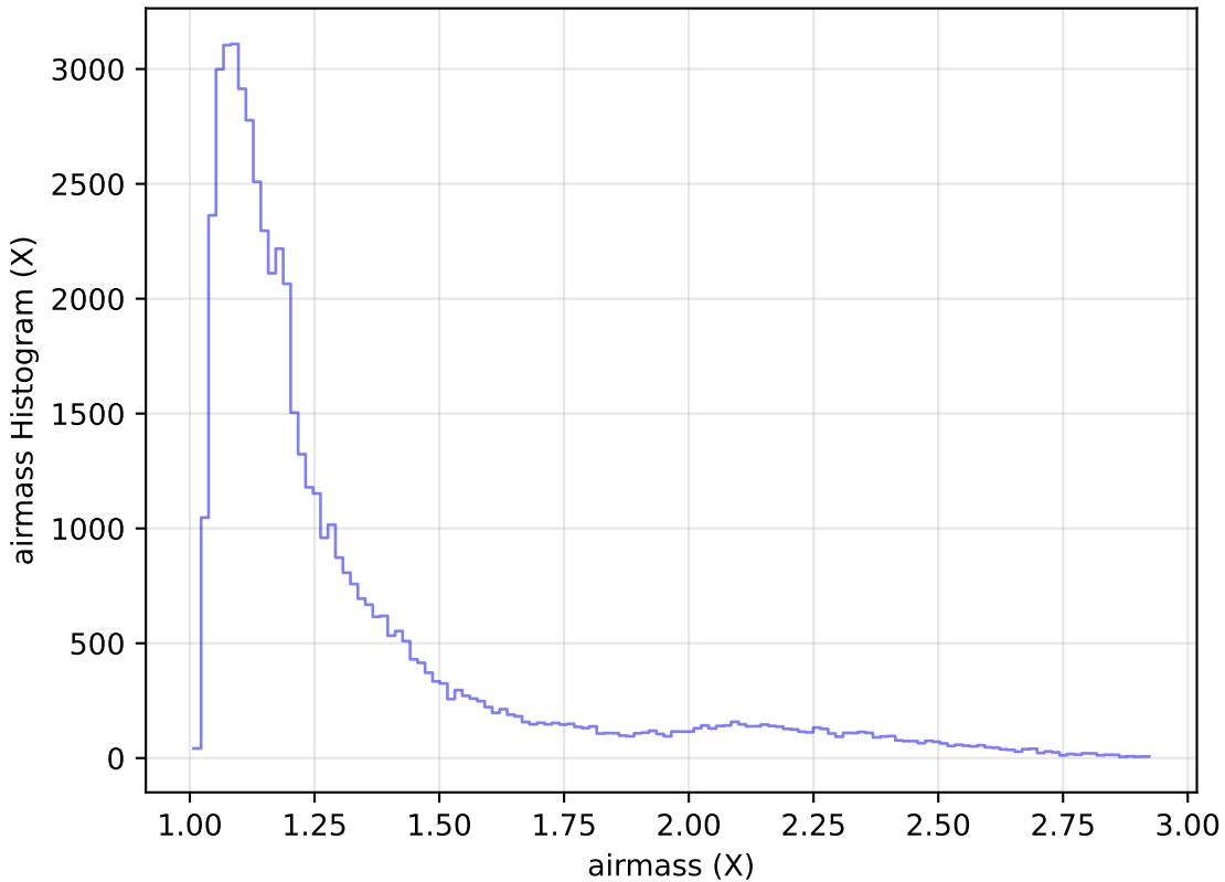
too_elab_heavy_r128_d3_gz_v3.4_10yrs Yr 1 i band: airmass Histogram
