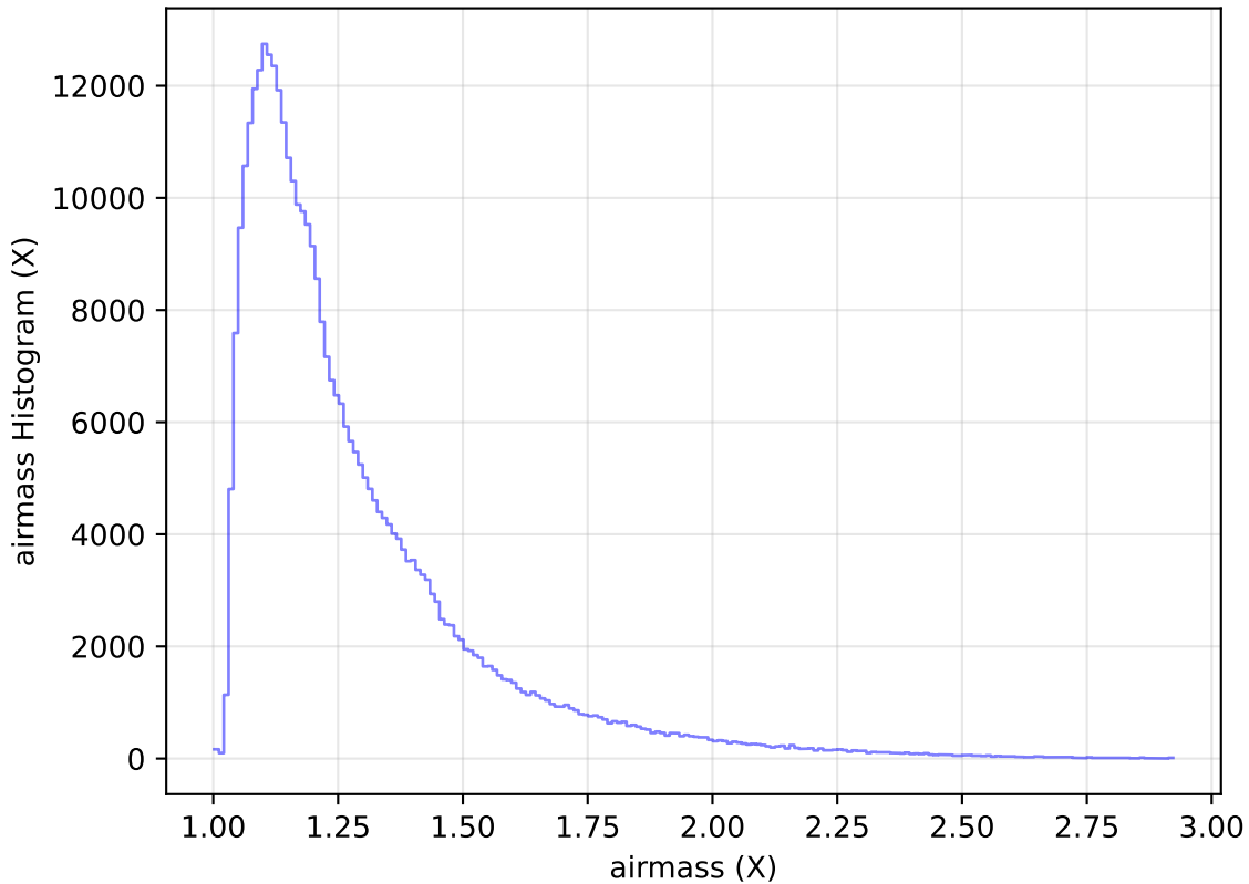
too_elab_heavy_r128_d3_gz_v3.4_10yrs WFD y band: airmass Histogram
