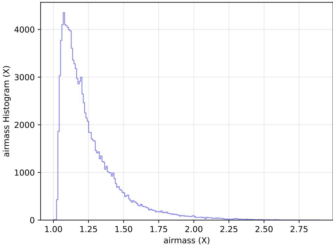
too_elab_heavy_r128_d3_gz_v3.4_10yrs WFD u band: airmass Histogram
