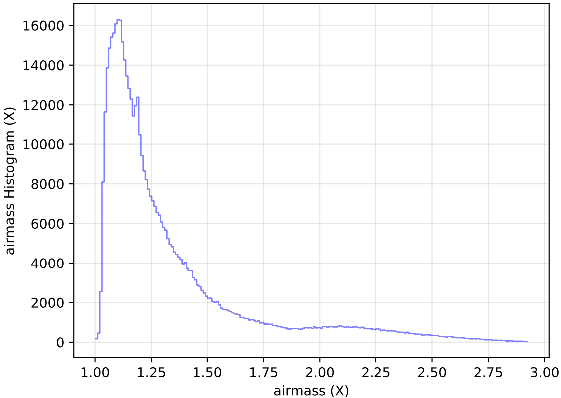
too_elab_heavy_r128_d3_gz_v3.4_10yrs WFD i band: airmass Histogram
