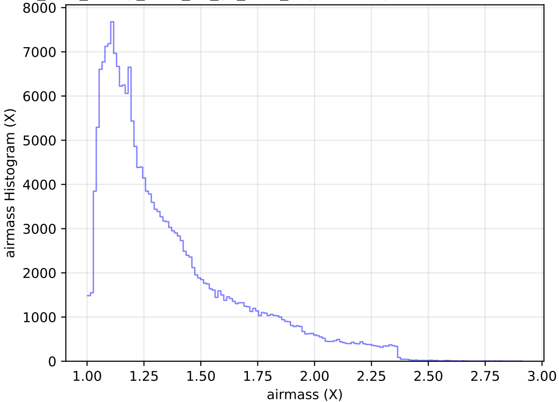
too_elab_heavy_r128_d3_gz_v3.4_10yrs WFD g band: airmass Histogram
