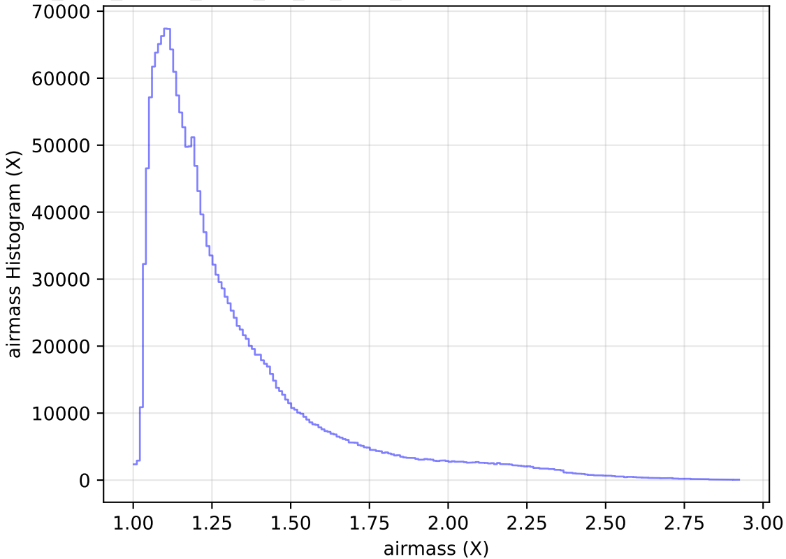
too_elab_heavy_r128_d3_gz_v3.4_10yrs WFD all bands: airmass Histogram
