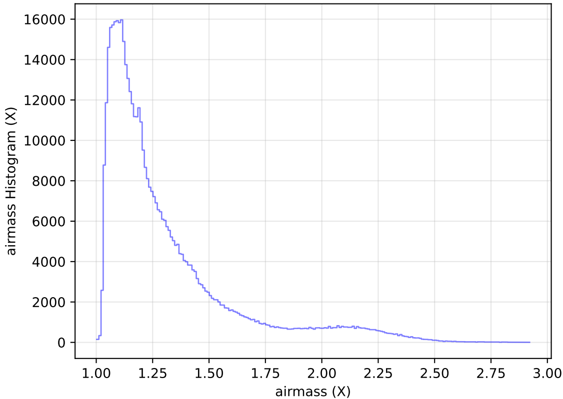
too_elab_heavy_r128_d3_gz_v3.4_10yrs All sky r band: airmass Histogram
