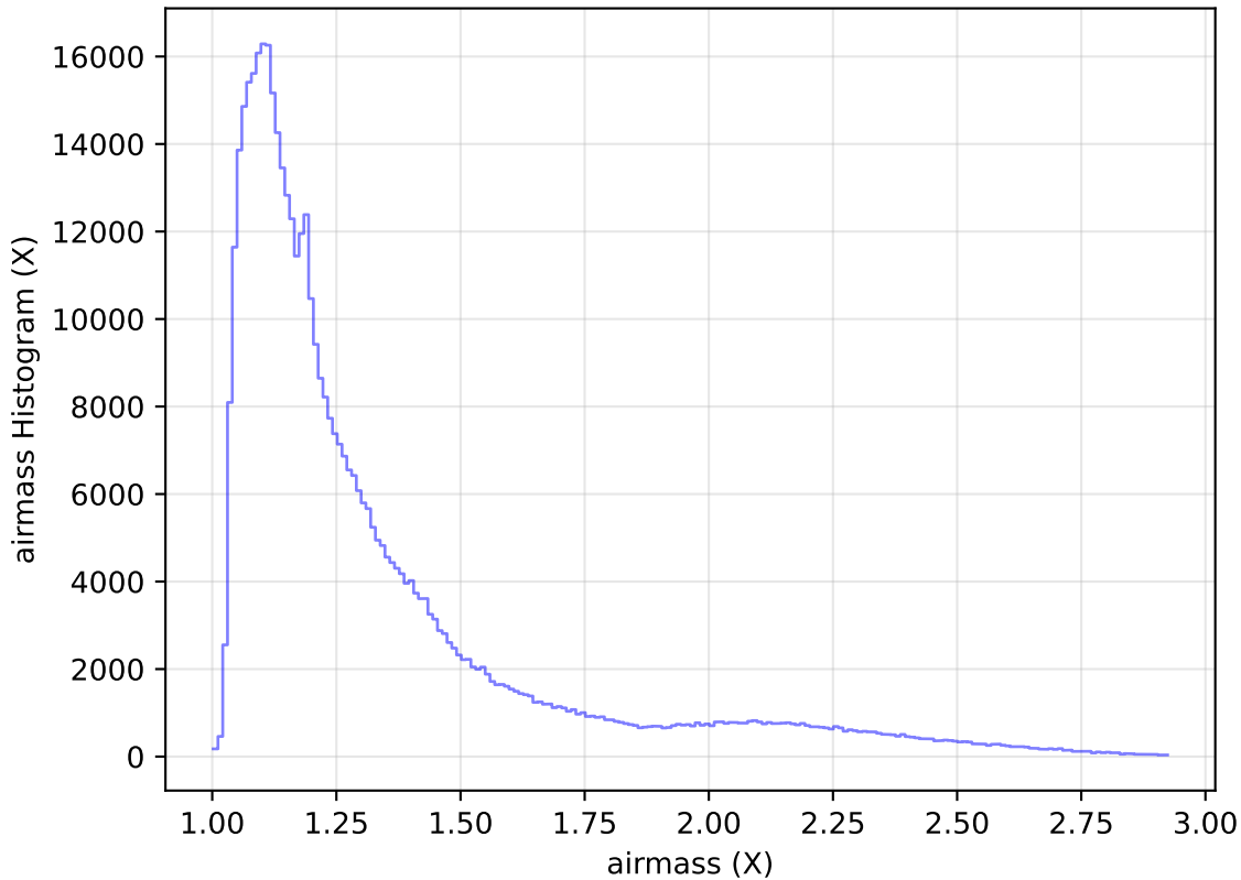
too_elab_heavy_r128_d3_gz_v3.4_10yrs All sky i band: airmass Histogram
