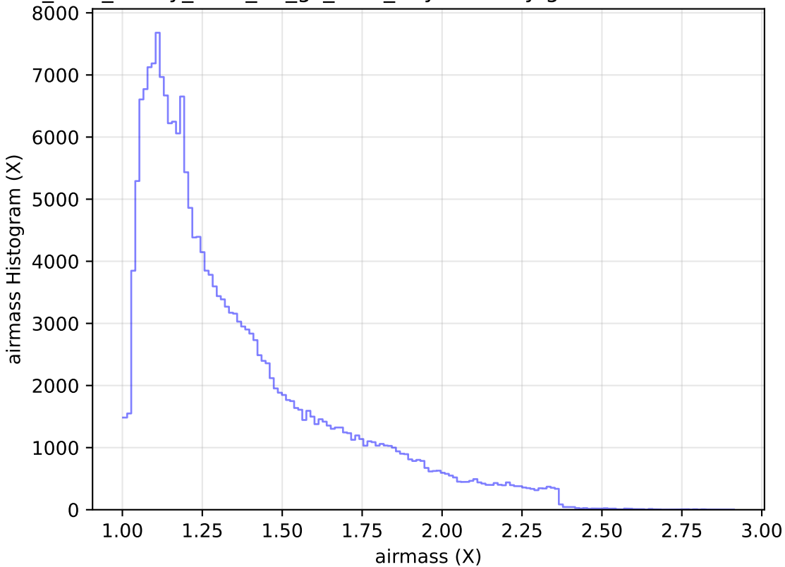
too_elab_heavy_r128_d3_gz_v3.4_10yrs All sky g band: airmass Histogram
