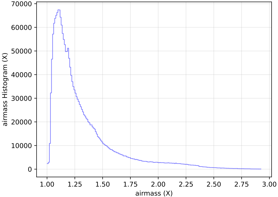
too_elab_heavy_r128_d3_gz_v3.4_10yrs All sky all bands: airmass Histogram
