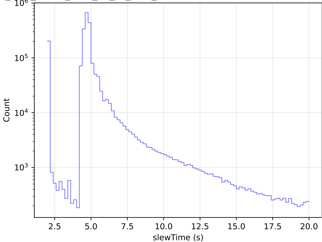
too_elab_heavy_r128_d3_gz_v3.4_10yrs All visits: Zoom Slew Time Histogram
