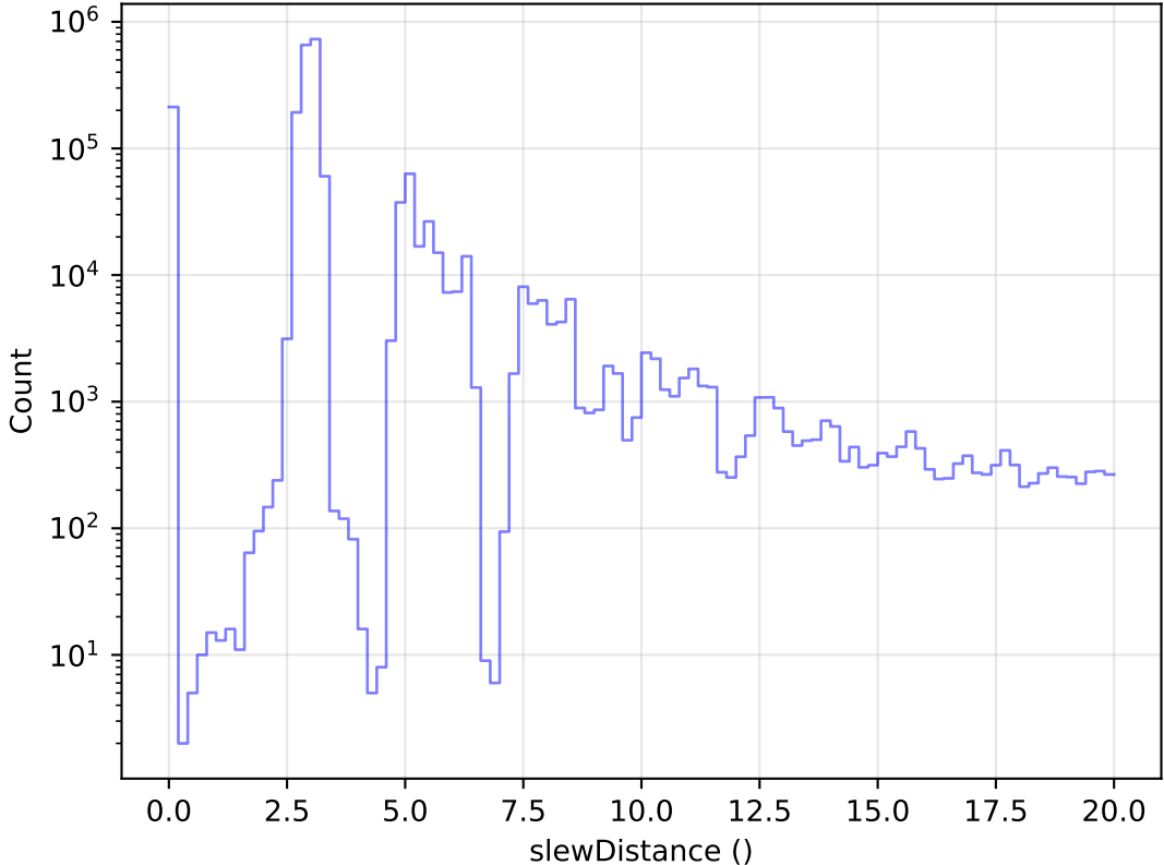
too_elab_heavy_r128_d3_gz_v3.4_10yrs All visits: Zoom Slew Distance Histogram
