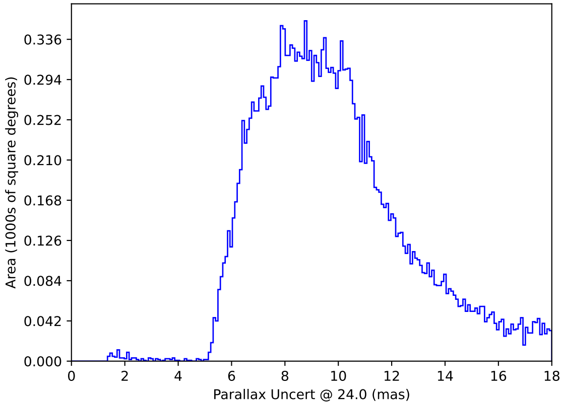
too_elab_heavy_r128_d3_gz_v3.4_10yrs All sky: Parallax Uncert @ 24.0
