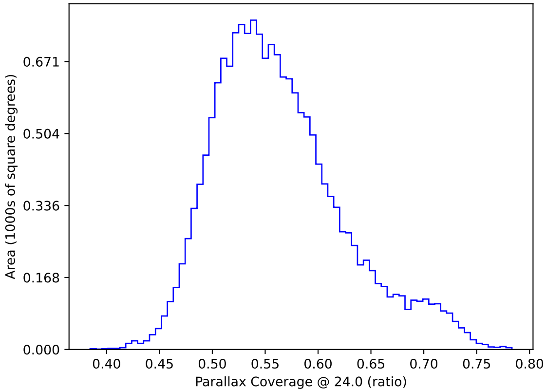
too_elab_heavy_r128_d3_gz_v3.4_10yrs WFD: Parallax Coverage @ 24.0
