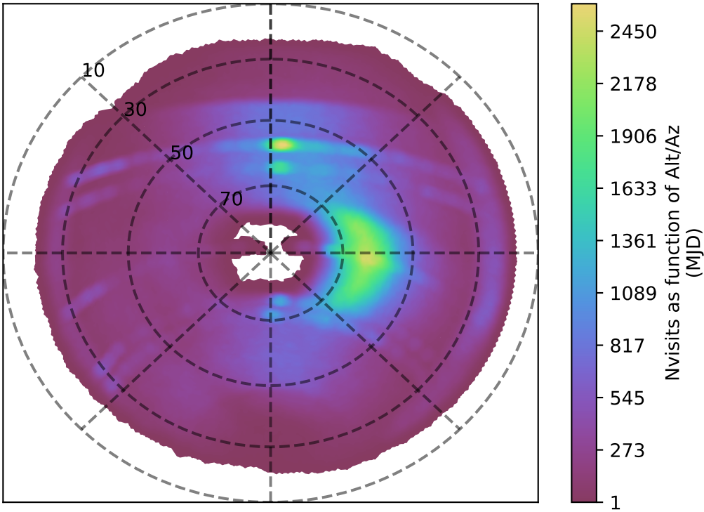
too_elab_heavy_r128_d3_gz_v3.4_10yrs i band: Nvisits as function of Alt/Az
