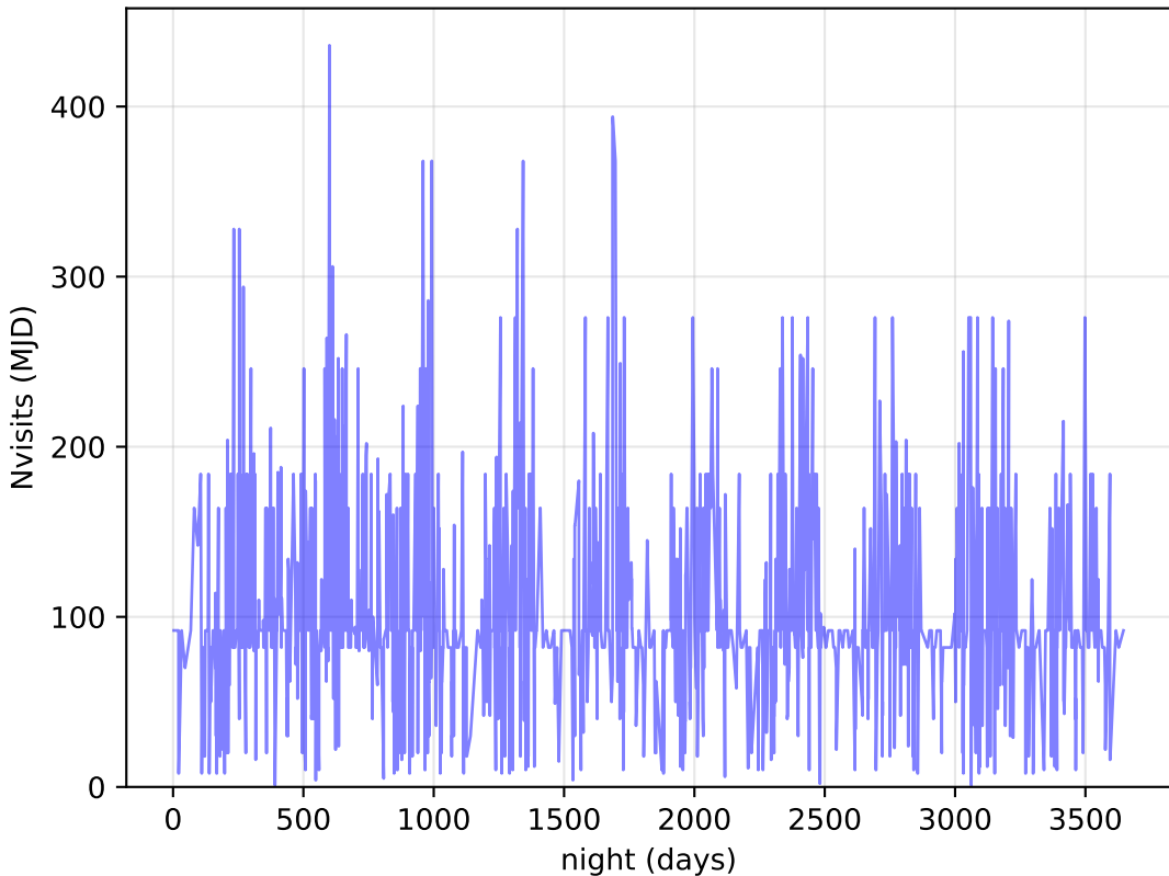
too_elab_heavy_r128_d3_gz_v3.4_10yrs DDF: Nvisits
