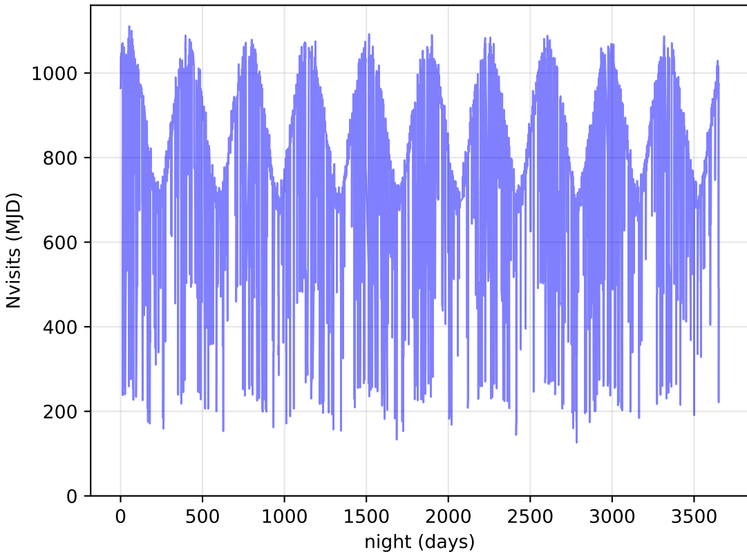
too_elab_heavy_r128_d3_gz_v3.4_10yrs All visits: Nvisits
