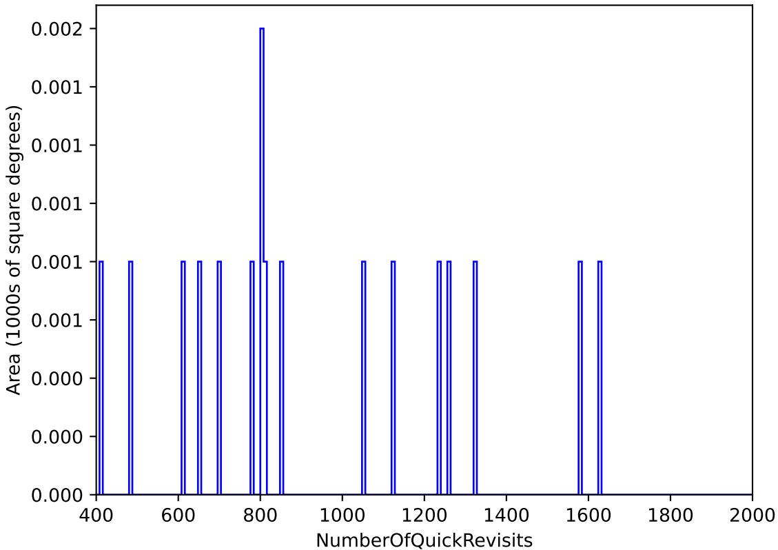
too_elab_heavy_r128_d3_gz_v3.4_10yrs WFD: NumberOfQuickRevisits
