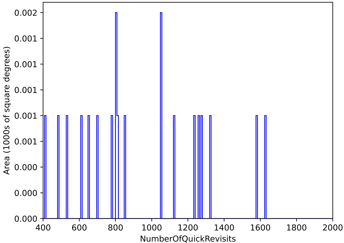
too_elab_heavy_r128_d3_gz_v3.4_10yrs All sky: NumberOfQuickRevisits
