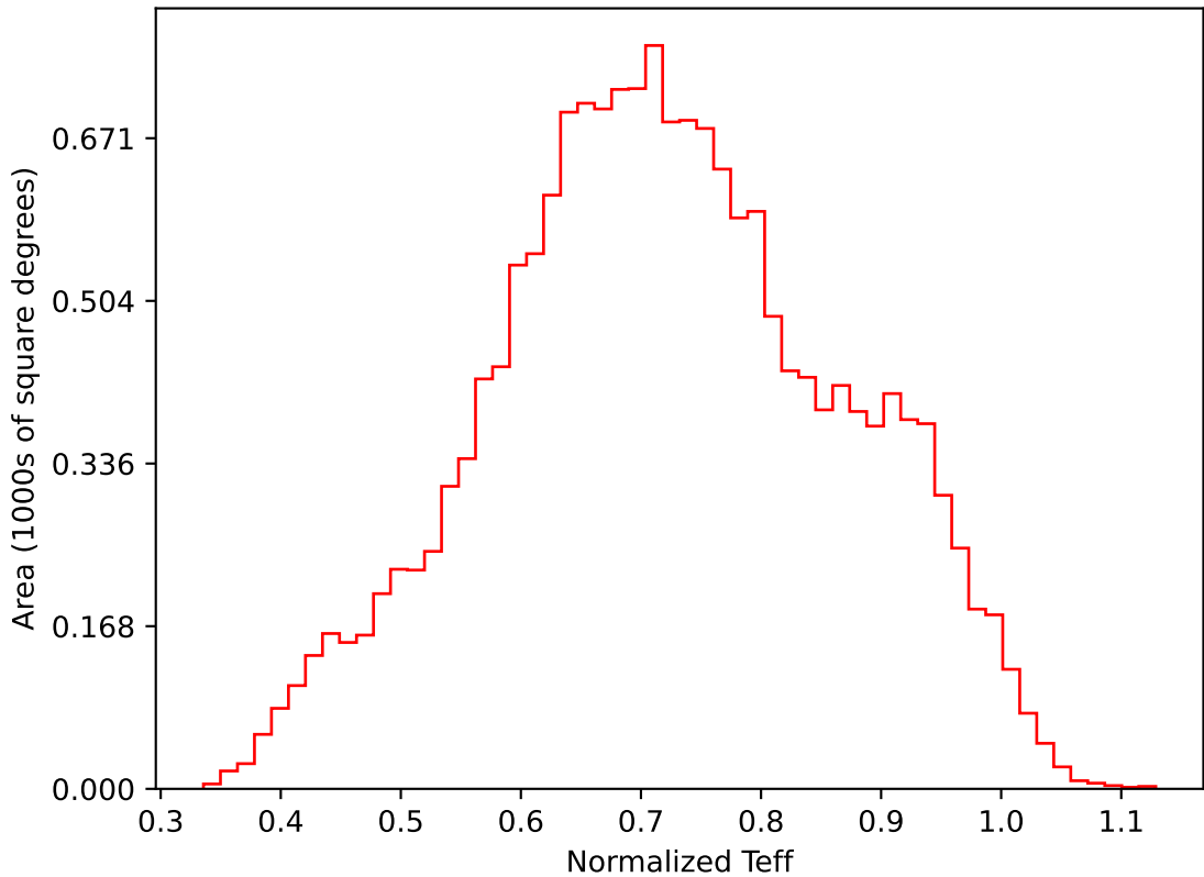
too_elab_heavy_r128_d3_gz_v3.4_10yrs WFD i band: Normalized Teff
