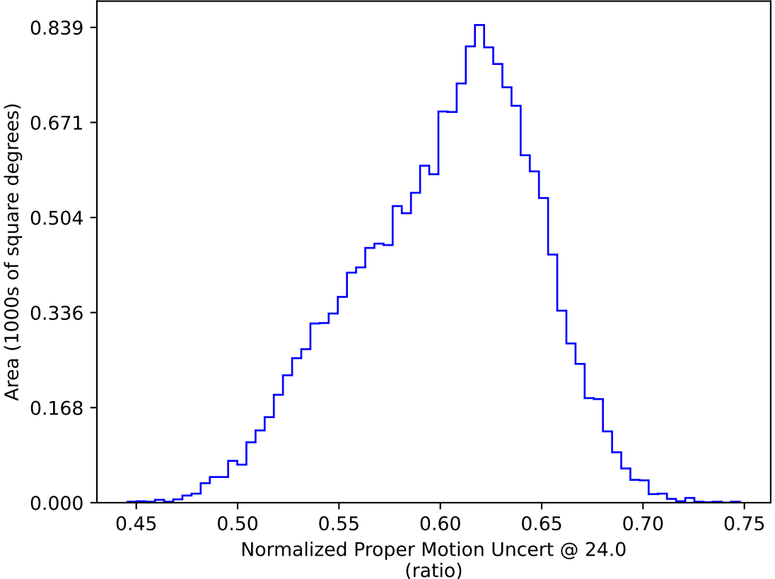
too_elab_heavy_r128_d3_gz_v3.4_10yrs WFD: Normalized Proper Motion Uncert @ 24.0
