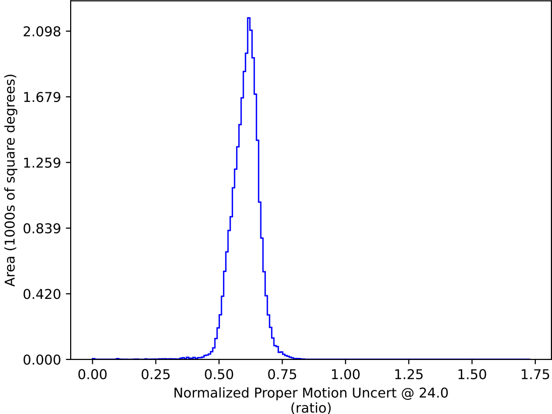
too_elab_heavy_r128_d3_gz_v3.4_10yrs All sky: Normalized Proper Motion Uncert @ 24.0
