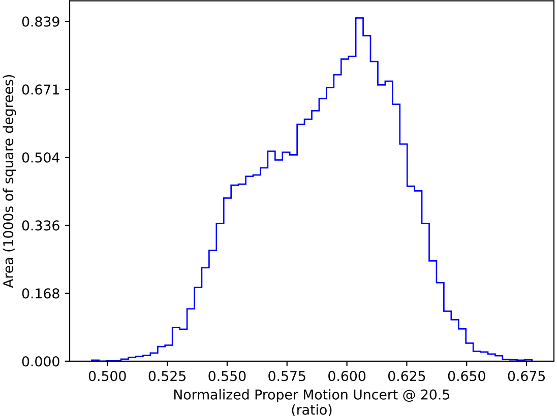
too_elab_heavy_r128_d3_gz_v3.4_10yrs WFD: Normalized Proper Motion Uncert @ 20.5
