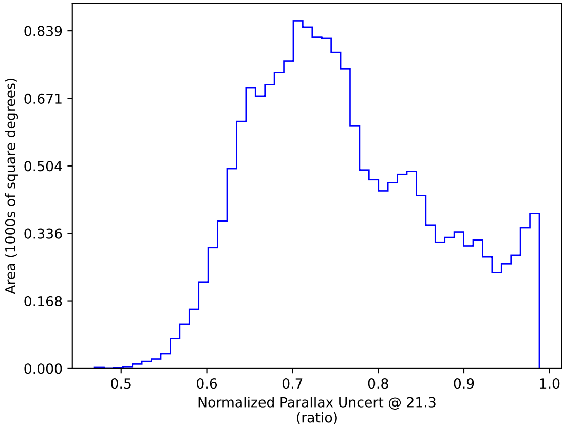
too_elab_heavy_r128_d3_gz_v3.4_10yrs WFD y band only: Normalized Parallax Uncert @ 21.3
