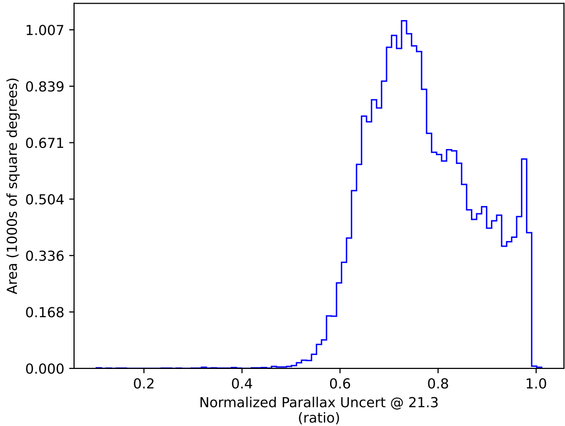
too_elab_heavy_r128_d3_gz_v3.4_10yrs All sky y band only: Normalized Parallax Uncert @ 21.3
