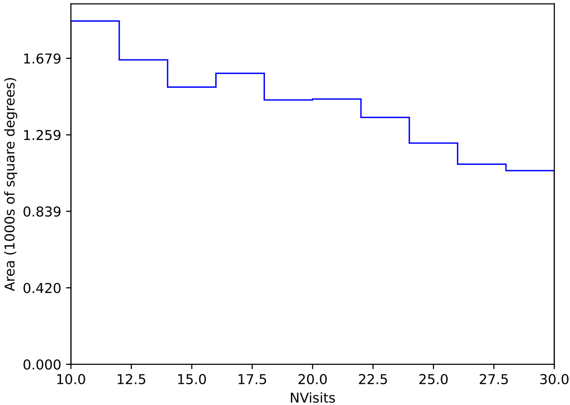
too_elab_heavy_r128_d3_gz_v3.4_10yrs Yr 3-4 y band: NVisits
