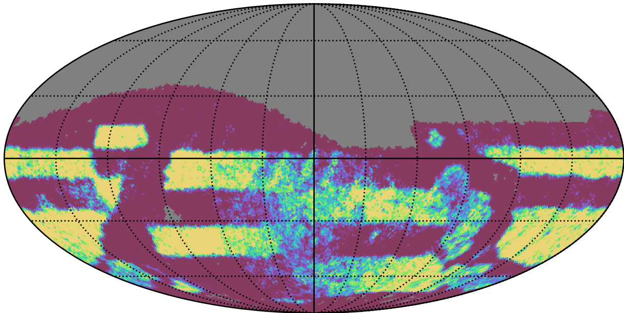
too_elab_heavy_r128_d3_gz_v3.4_10yrs Yr 3-4 r band: NVisits
