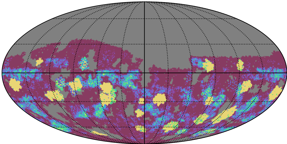
too_elab_heavy_r128_d3_gz_v3.4_10yrs Yr 3-4 g band: NVisits
