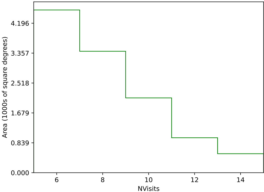
too_elab_heavy_r128_d3_gz_v3.4_10yrs Yr 3-4 g band: NVisits
