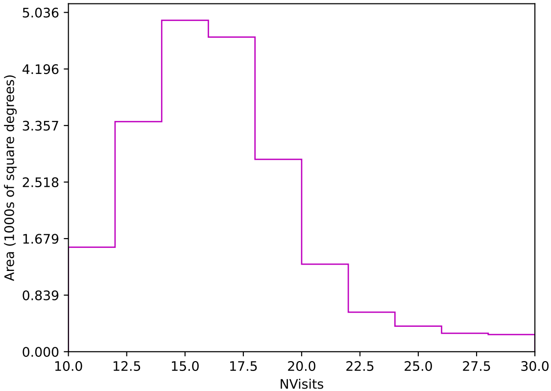
too_elab_heavy_r128_d3_gz_v3.4_10yrs Yr 1 z band: NVisits
